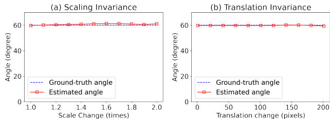
Fig. 1: Invariance property of the rotation estimation: When estimating the rotation angle between two images, the difference in image scale or translation have minor effect on the results.
